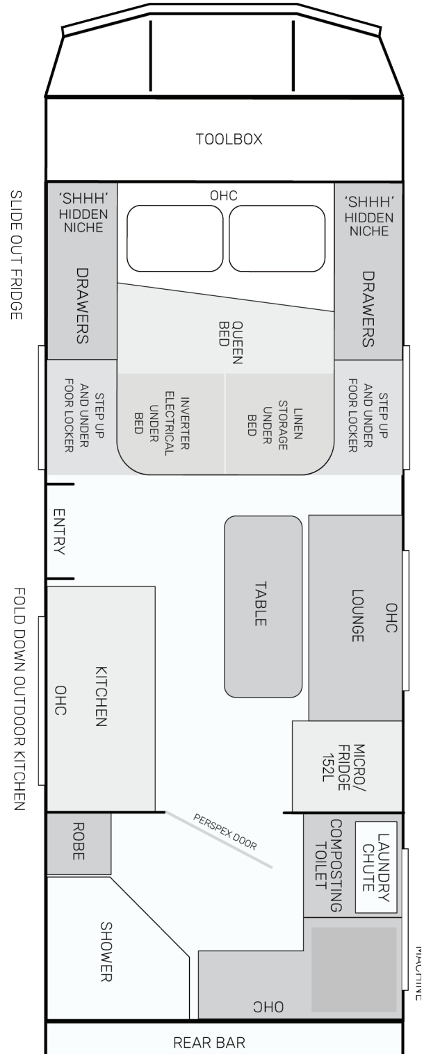
TOOLBOX LAYOUT (OPTIONAL UPGRADE) THE VAN WILL BE 350MM LONGER WITH THE TOOLBOX
