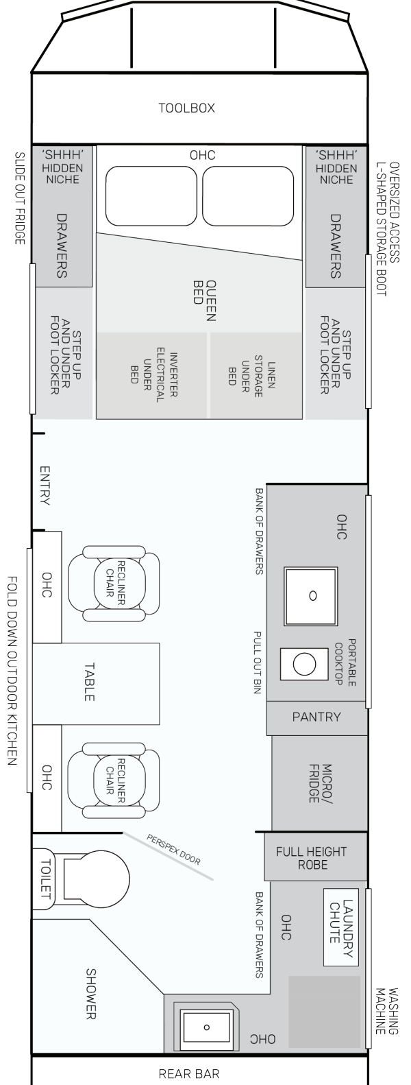
TOOLBOX LAYOUT (OPTIONAL UPGRADE)
