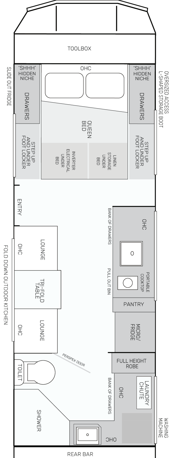
TOOLBOX LAYOUT (OPTIONAL UPGRADE) THE VAN WILL BE 350MM LONGER WITH THE TOOLBOX
